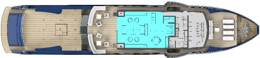
UPPER DECK
